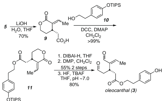
Scheme 3. Synthesis of ( \pm )-oleocanthal.
